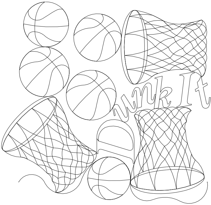
Basketball E2E
